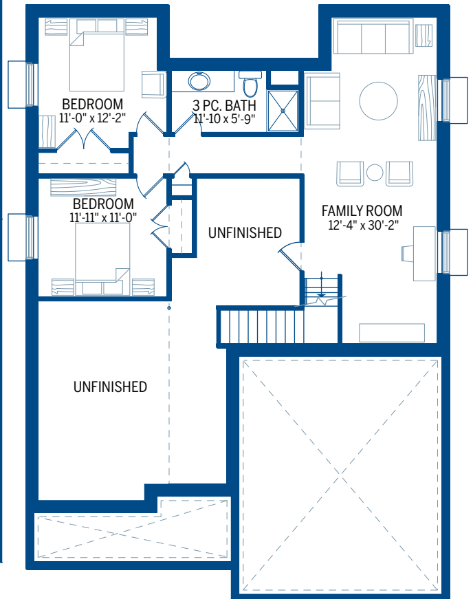
Optional Lower Level Plan 920 sq.ft.
