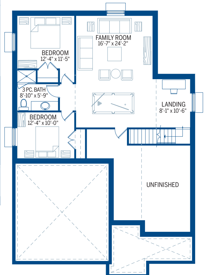
Optional Lower Level Plan 1009 sq.ft.
